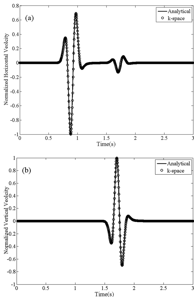
FIG. 4. Velocity components time-series at the receiver for the example of an explosive source above a fluid-solid interface (Sec. IV B). Analytical solution (solid), k -space method (circles). (a) Horizontal particle velocity. (b) Vertical particle velocity.
