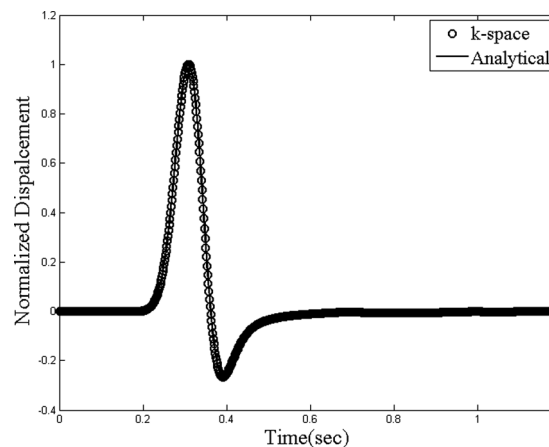
FIG. 2. The radial displacement as a function of time 400 m from an explosive source in a 2D homogenous elastic medium (i.e., cylindrical wave propagation). Analytical solution (solid), k -space method (circles).
