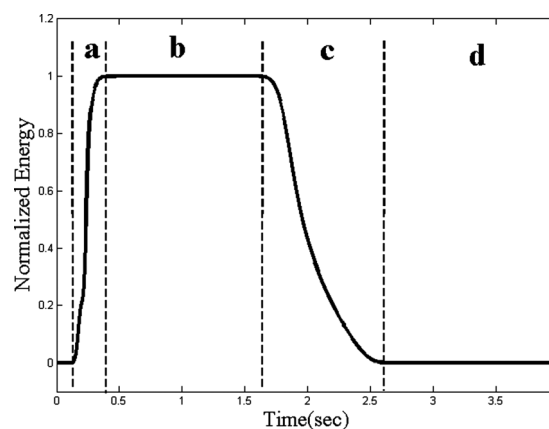
FIG. 3. The net energy of the propagating wave vs time. After the source is added to the field [region (a)], the energy is preserved [region (b)] until the wave reaches the PML [region (c)], where it is attenuated, after which gradually there is no energy remaining in the domain [region (d)].
