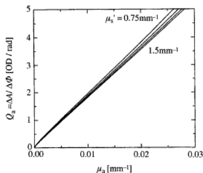
Figure 6. The predicted change in the ratio Q_a (= (\partial A/\partial \mu_a)/(\partial \Phi/\partial \mu_a)) for measurements across 3 cm of tissue as a function of \mu_a for a range of different \mu'_s values (Kohl et al. 1996).
