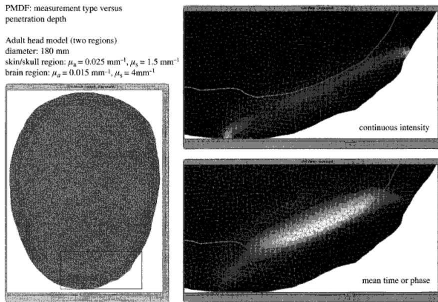
Figure 7. Continuous intensity and mean time PMDFs estimated for light travelling through the adult head. The data was calculated using a finite element implementation of the time-dependent diffusion equation, the source-detector spacing being 4.5 cm.
