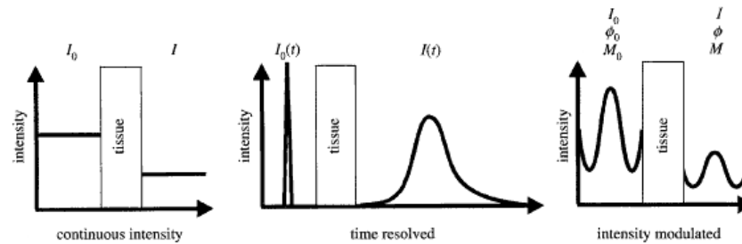
Figure 3. Schematic illustration of the three main types of NIRS instrumentation.
